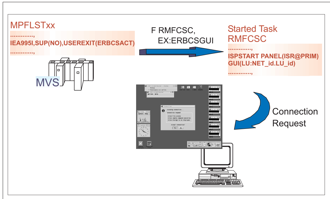
Figure 80. RMFCS Scenario I: Message-Initiated Monitoring
